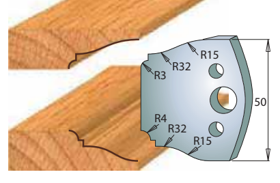
Pair of knives 690.568 Pair of limiters 691.568
