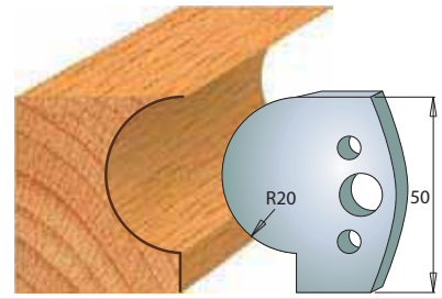
Pair of knives 690.562 Pair of limiters 691.562
