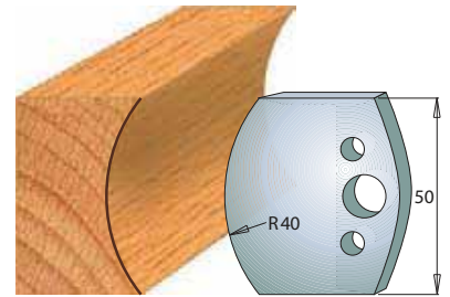
Pair of knives 690.553 Pair of limiters 691.553
