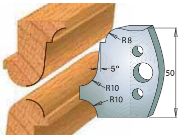
Pair of knives 690.557 Pair of limiters 691.557
