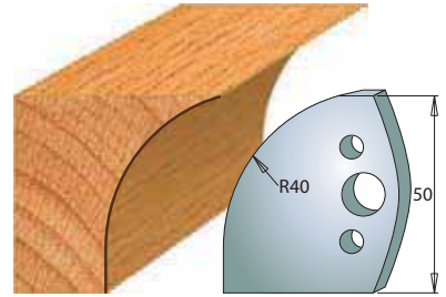
Pair of knives 690.565 Pair of limiters 691.565
